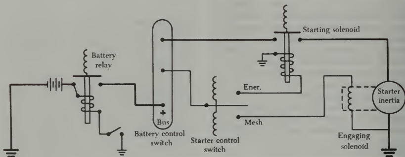
FIGURE 5-2. Electric inertia starting circuit.
